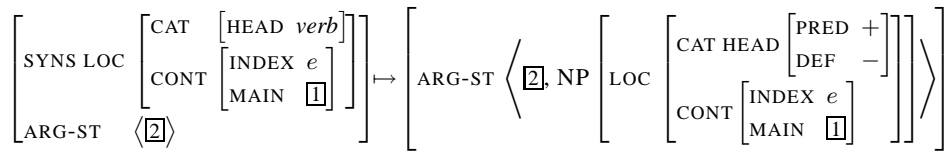
Figure 4: Description resulting from combining the constraints on coc-lr and part-event-coc-lr
